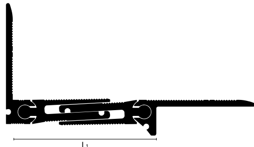
Illustrated scale dimension 1:2 (GADP 700 AN)
