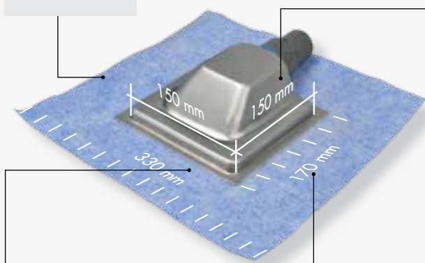
330x330 mm Membrane size in the model SQUAREDRAIN SDS150IL/M
